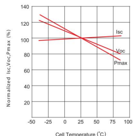
Temperature Dependence of Isc, Voc, Pmax
