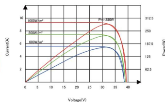
Current-Voltage-Power-Voltage Curve (280W)
